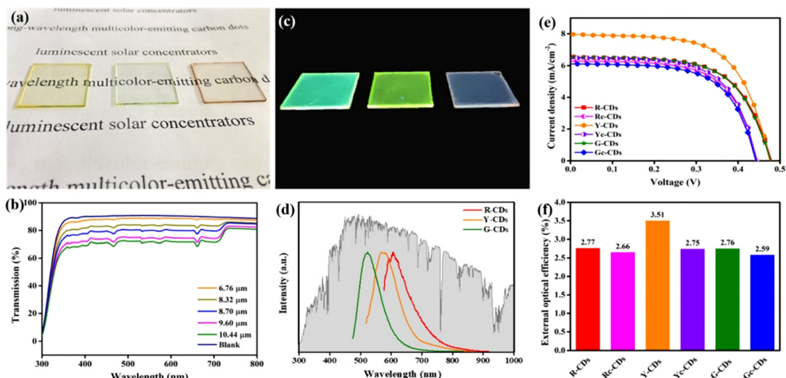
Fig. 11 (a) Photographs of the R, Y, G C-dot-based LSCs under daylight. (b) Transmittance spectra of Y CD-based LSCs with different thicknesses (0.32 wt% of C-dots concentration). (c) Photographs of the R, Y, G C-dot-based LSCs under UV light. (d) Emission spectra of the R, Y, G C-dot-based LSCs. (e) Relationship of the photocurrent density and photovoltage ( J-V ) of the various C-dot-based LSCs (0.32 wt% of C-dot concentration, 9.6 \mu\text{m} of thickness). (f) External optical efficiencies of the various C-dot-based LSCs (0.32 wt% of C-dot concentration, 9.60 \mu\text{m} of thickness). Reproduced with permission from ref. 50. Copyright 2020, American Chemical Society.
