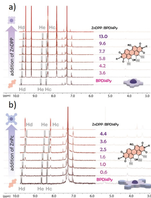
Fig. 5 (a) 1 H NMR spectra in CDCl 3 of a titration of BPDIC7 solution (0.5 mL, 0.055 mM) with increasing amounts of ZnDPP (400 μL, 13 mM) in CDCl 3 . and (b) ZnPc (180 μL, 0.13 mM) in CDCl 3 .
