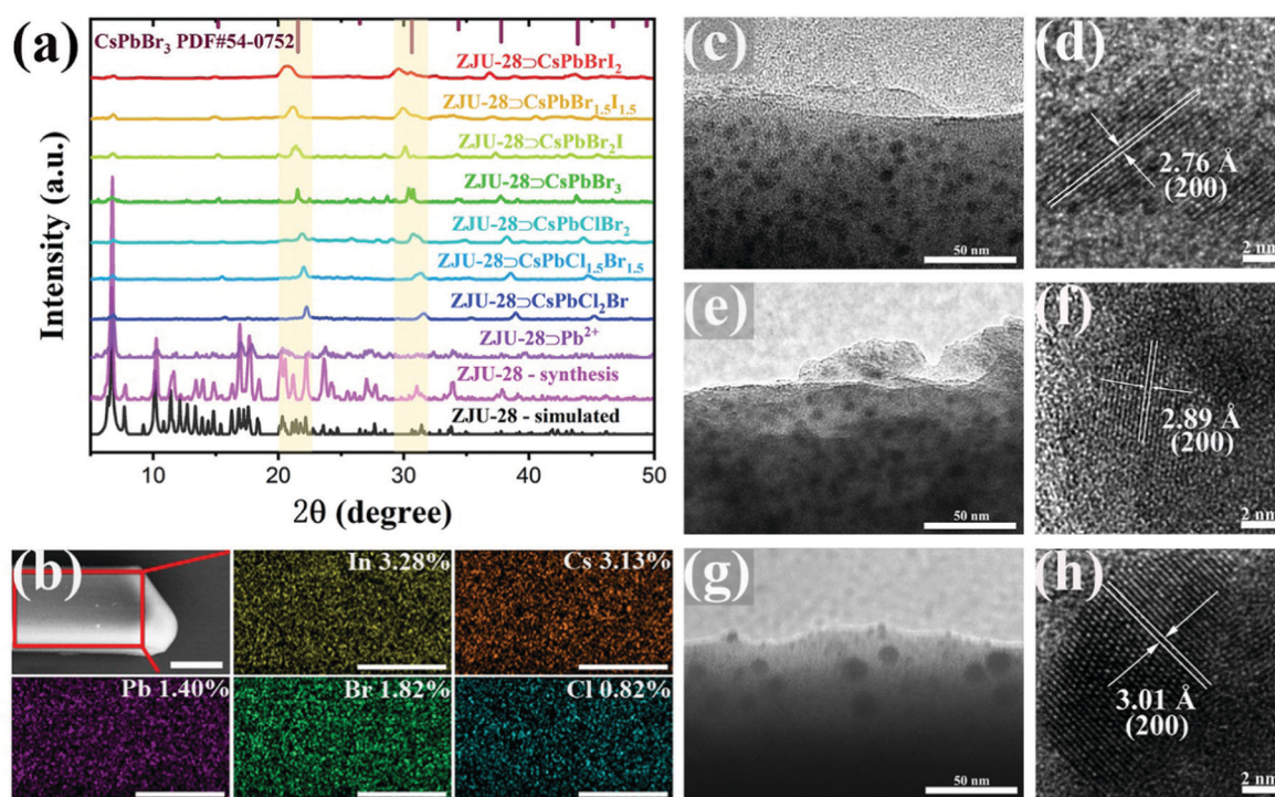
Fig. 1 (a) PXRD patterns of ZJU-28, \text{ZJU-28} \supset \text{Pb}^{2+} and \text{ZJU-28} \supset \text{CsPbX}_3 crystals. (b) The SEM image of \text{ZJU-28} \supset \text{CsPbClBr}_2 and the corresponding elemental mapping diagrams of In, Cs, Pb, Cl, and Br. Scale bar, 5 \mu\text{m} . TEM image and HR-TEM image of (c and d) \text{ZJU-28} \supset \text{CsPbClBr}_2 , (e and f) \text{ZJU-28} \supset \text{CsPbBr}_3 and (g and h) \text{ZJU-28} \supset \text{CsPbBrI}_2 .
