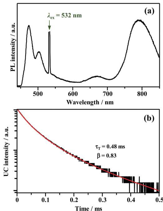
Fig. 4 (a) PL spectrum obtained for the deaerated THF solution of Au 2 Cu 6 (11 μM) and perylene (5 mM), and (b) decay curve of the upconverted emission of perylene obtained by monitoring only the λ ≤ 492 nm region using short-pass filters. The fitting of the decay curve was performed using eqn (1). The 532 nm-CW laser was used in these measurements. Note that the upconverted emission of perylene was also observed when using a 640 nm-CW laser.
