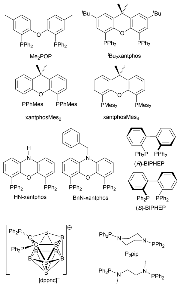
Scheme 10 Structures of wide-bite angle bis(phosphanes) used in [\text{Cu}(\text{P}^{\wedge}\text{P})(\text{N}^{\wedge}\text{N})]^+ complexes. See Scheme 1 for POP and xantphos.
