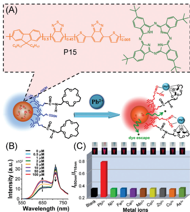
Fig. 6 (A) Schematic diagram of the construction of the CP-based Pb^{2+} sensing probe. (B) Emission spectra of Pdts under different concentrations of Pb^{2+} . The concentration range of Pb^{2+} is 0 to 100 \mu M ( \lambda_{ex} = 450 nm), disposed with 20 nM Pdts at pH 7.4. (C) The effect of different ionic species (50 \mu M ) on the luminescence intensity of Pdts solution. Inset: each sample under bright field (upper row) and UV light at 365 nm (lower row). Reproduced with permission from ref. 72. Copyright 2015 American Chemical Society.
