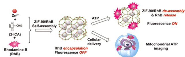
Fig. 8 Schematic representation of modulating the host-guest chemistry of nanoscale RhB/ZIF-90 for fluorescent ATP sensing and mitochondrial ATP imaging. Reproduced with permission. 56 Copyright 2017, American Chemical Society.
