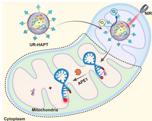
Fig. 3 Schematic illustration of the design of UR-HAPT for precise imaging of subcellular enzymatic dynamics of APE1 during NIR light-mediated, mitochondria-targeted PDT. 40 Copyright 2022, Wiley-VCH GmbH.
