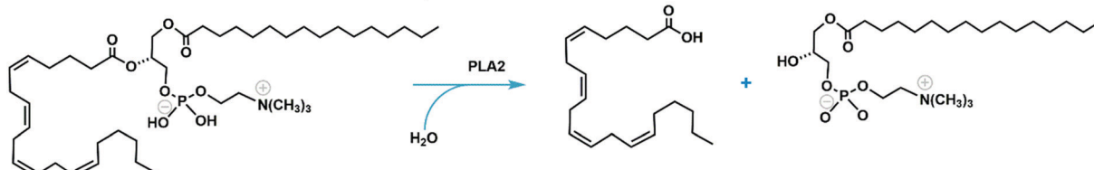
Fig. 1 The hydrolysis mechanism of sPLA2.
