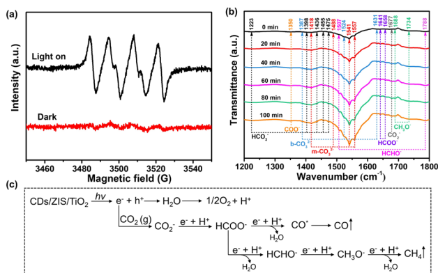
Fig. 7 (a) ESR spectra of DMPO \cdot O_2^- on 5-CDs/ZIS/TiO 2 . (b) In situ DRIFTS spectra of surface adsorbed CO_2 species and photocatalytic CO_2 reduction intermediates on 5-CDs/ZIS/TiO 2 . (c) Photocatalytic reaction pathways over CDs/ZIS/TiO 2 .
