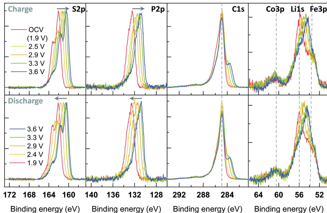
Fig. 29 Operando XPS experimental results during potentiostatic measurement of a working electrode made of 45 wt% LCO, 50 wt% amorphous (\text{Li}_2\text{S})_3\text{-P}_2\text{S}_5 and 5 wt% VGCF cycled vs. \text{InLi}_x . Reprinted from ref. 182.
