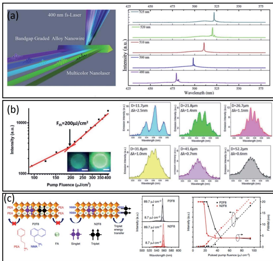
Fig. 4 (a) Schematic representation of optical pumping lasing experiments with a 400 nm fs-laser ( \sim 40 fs, 10 kHz) as the excitation source. Typical lasing spectra obtained from a single CsPbCl 3-3x Br 3x alloy nanowire at a high pump density. Reproduced with permission from ref. 80, Copyright 2020 The Royal Society of Chemistry. (b) Emission intensity versus excitation fluence measured from a CsPbBr 3 QD microdisk and lasing spectra of QD microdisks with D = 11.7, 21.8, 26.7, 31.8, 41.6 , and 52.2 \mu\text{m} , respectively. \Delta\lambda is the average "mode spacing" of the observed longitudinal cavity modes. Reproduced with permission from ref. 83, Copyright 2018 WILEY-VCH Verlag GmbH & Co. KGaA, Weinheim. (c) Chemical structures and evolution of emission spectra under pulsed excitation (3 ns) with different pump fluences. Photoluminescence, ASE and FWHM as a function of the pump fluence for a CW perovskite laser. Reproduced with permission from ref. 87, Copyright Springer Nature SharedIt.
