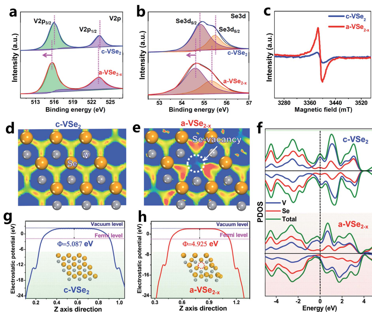
Fig. 2 (a) XPS V 2p spectra of c\text{-VSe}_2 and a\text{-VSe}_{2-x} . (b) XPS Se 3d spectra of c\text{-VSe}_2 and a\text{-VSe}_{2-x} . (c) EPR spectra of c\text{-VSe}_2 and a\text{-VSe}_{2-x} . (d and e) Electron localization function images of c\text{-VSe}_2 and a\text{-VSe}_{2-x} . Blue and red regions represent the electron depletion and accumulation, respectively. (f) PDOS of c\text{-VSe}_2 and a\text{-VSe}_{2-x} . (g and h) Average potential profiles of c\text{-VSe}_2 and a\text{-VSe}_{2-x} .
