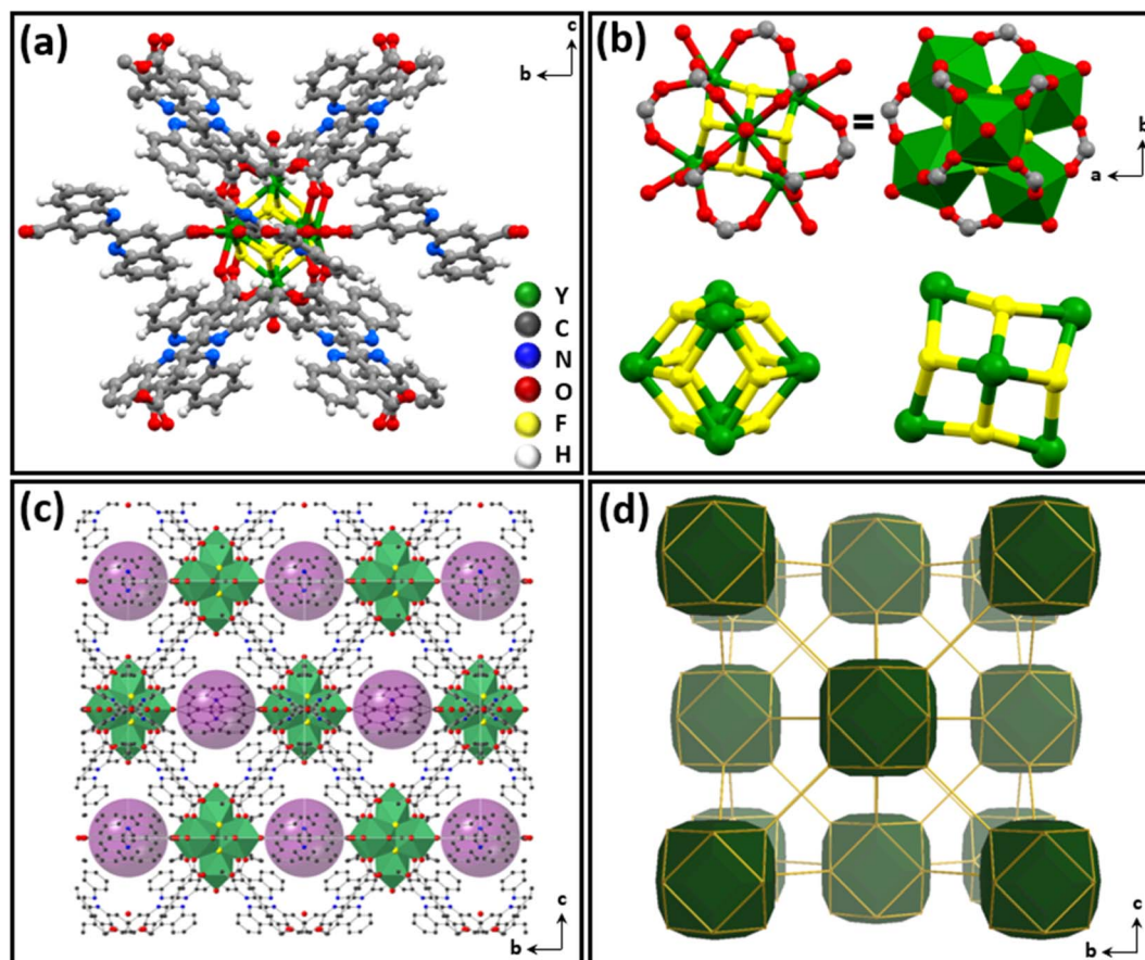
Fig. 4 Crystal structure of Y-BCA-3D (a) cluster structure with hexanuclear node, (b) c-axis view of hexanuclear and isolated Y_6F_8 cluster, (c) extended 3D network view along the a -axis showing 6.3 Å spherical cavities (purple), and (d) underlying net topology of the MOF viewed along the a -axis.
