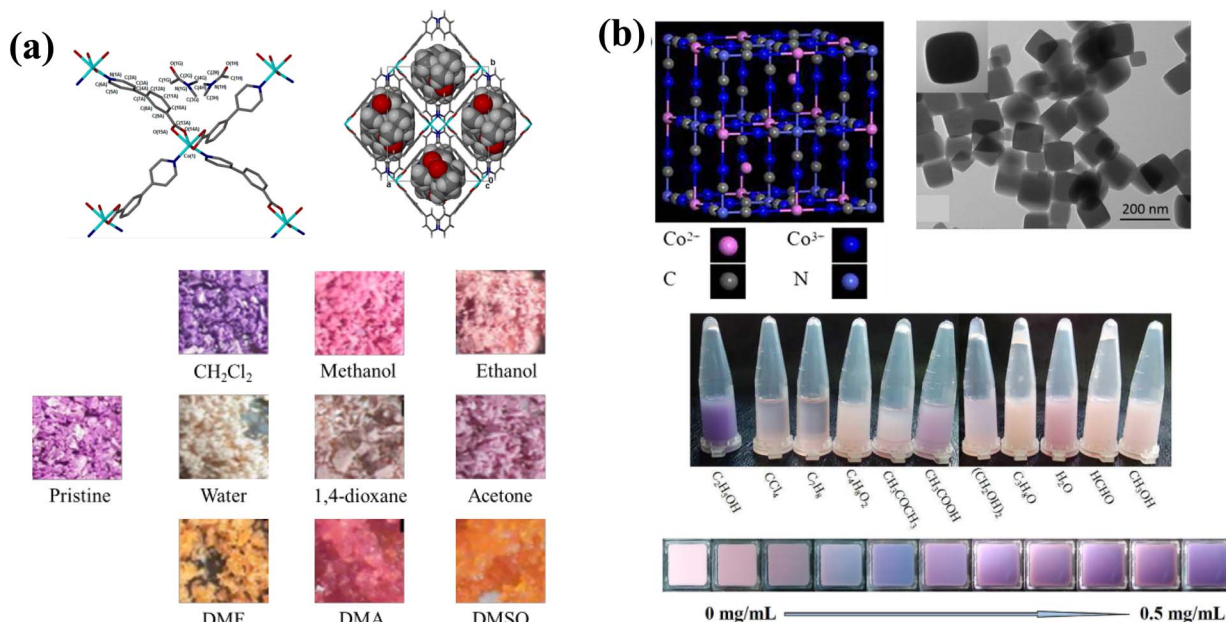
Fig. 3 (a) Coordination environment of Co(II), packing of [\text{Co}(\text{3,4pba})_2 \cdot (\text{H}_2\text{O})] \cdot 1/2\text{DMF} \cdot \text{H}_2\text{O}]_n and pictures of powdered samples after exposure to different solvents. Figures adapted from ref. 126. (b) Structure of \text{Co}_3[\text{Co}(\text{CN})_6]_2 and TEM image of the nanoparticles; the colour of \text{Co}_3[\text{Co}(\text{CN})_6]_2 films changes from pink to purple gradually with an increasing ethanol concentration gradient. Adapted with permission from ref. 96.
