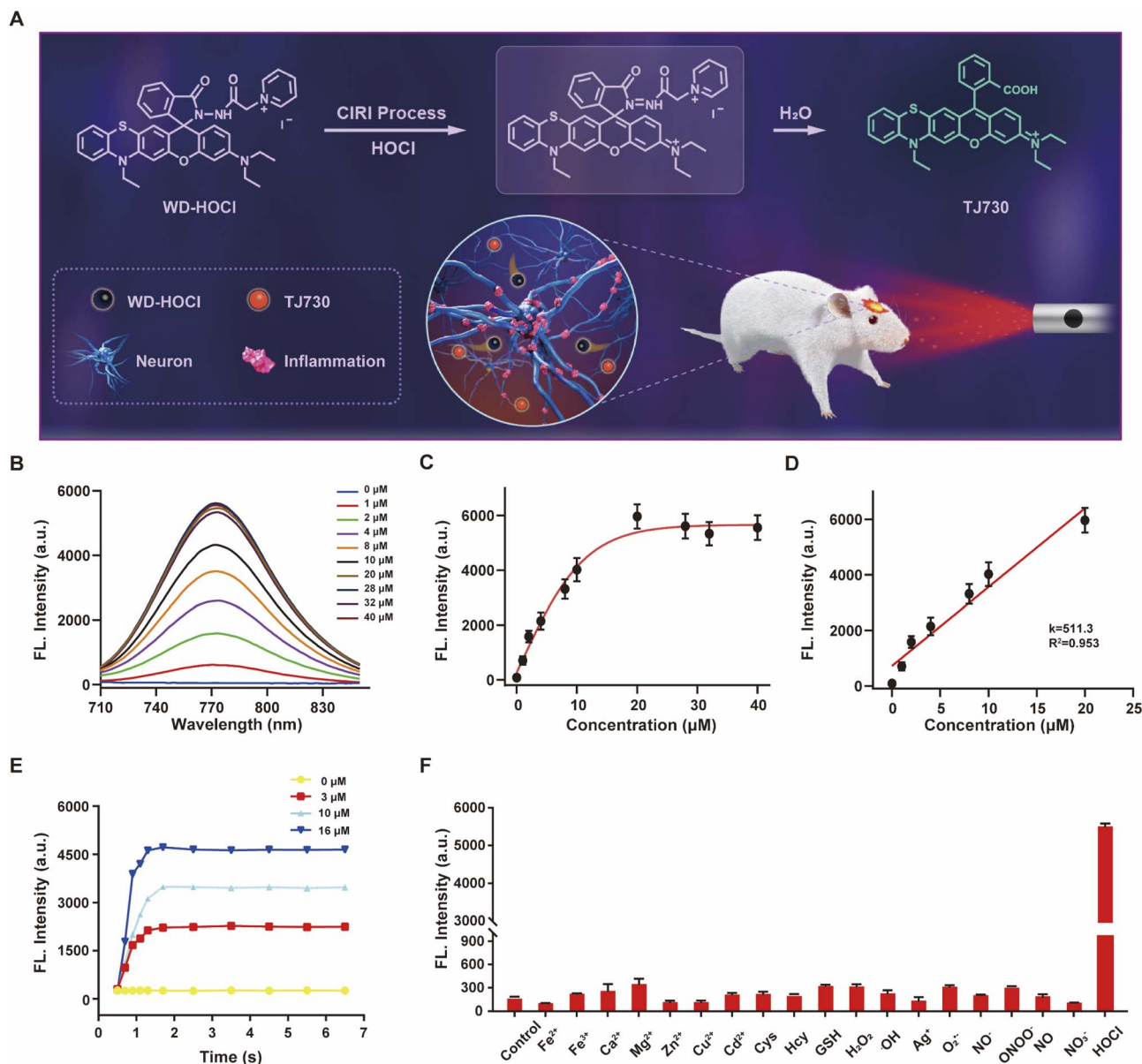
Fig. 2 (A) Recognition mechanism of WD-HOCl . (B) Fluorescence spectra for WD-HOCl upon exposure to different amounts of HOCl (0–40 μM). (C) Fluorescence intensity of WD-HOCl at 762 nm as a function of the HOCl concentration. (D) Linear fluorescence response of WD-HOCl toward HOCl (0–20 μM). (E) Time-dependent reaction profiles of 10 μM WD-HOCl and (0, 3, 10, and 16 μM) HOCl. (F) Fluorescence responses of WD-HOCl to a blank control (a), 20 μM metal ions ((b–i) Fe 2+ , Fe 3+ , Ca 2+ , Mg 2+ , Zn 2+ , Ag + , Cu 2+ , and Cd 2+ , respectively), 1.0 mM biomolecules ((j–l) Cys, Hcy, and GSH, respectively), 100 μM ROS ((m–o), H 2 O 2 , ·OH, and O 2 ·- , respectively), 100 μM reactive nitrogen species (RNS, (p–s) NO 2 - , ONOO - , NO, and NO 3 - , respectively), and 20 μM HOCl.
