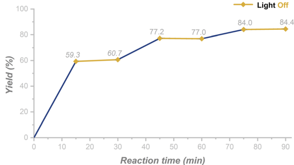
Fig. 1 Light on-off experiments for the synthesis of N -OH oxindole (the reaction was performed in a sealed NMR tube and NMR yields were shown, ESI 5.3†).
