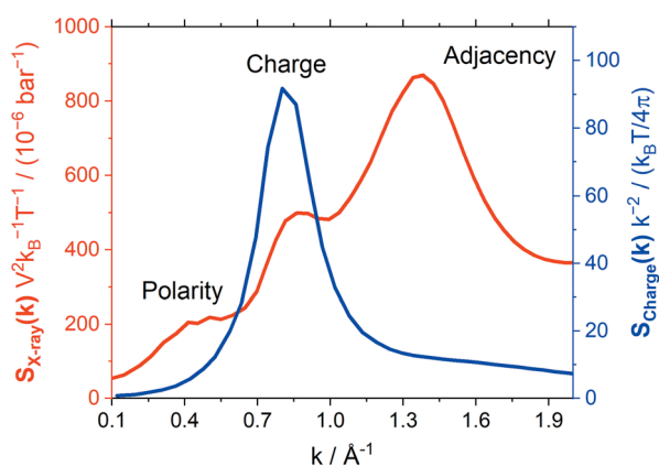
Fig. 11 Structure factors obtained from the MD simulation of [C 4 C 1 im][NTf 2 ] at 298 K. The red curve corresponds to S_{\text{X-ray}} measured in a SAXS experiment, the blue curve is the charge–charge correlation structure factor S_{\text{charge}} . Here, S_{\text{X-ray}} is normalised by \left(\sum_i f_i(\vec{k})\right)^2 .
