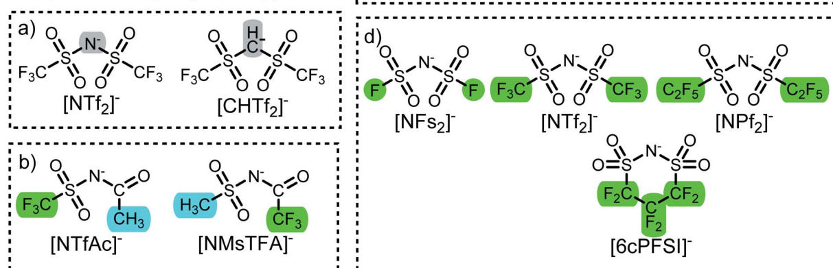
Fig. 2 Targeted modifications of the [NTf 2 ] − anion investigated in this work. Tf = triflate, Ac = acetyl, TFA = trifluoroacetyl, Ms = methanesulfonyl, FS = fluorosulfonyl, Pf = pentafluoroethylsulfonyl.
