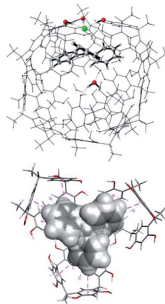
Fig. 3 The most stable structure of ionized trityl chloride inside the hexameric resorcinarene capsule ( \text{Tr}^+ \cdot \text{Cl}^- @ \text{C}_6\text{M} ). (Top) Balls and sticks refer to the QM level. (Bottom) Bottom view regarding the plane that cuts the capsule parallel to the trityl cation longitudinal axes; the dots and dashed-lines in purple refer to \text{CH}-\pi interactions.
