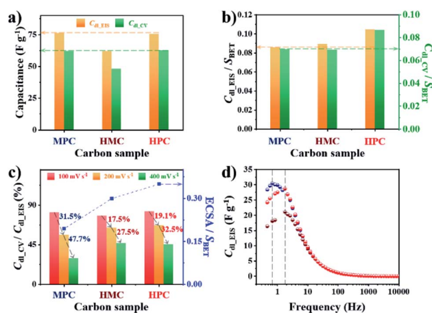
Fig. 2 (a) Electric double layer capacitance calculated from EIS measured at OCP ( C_{\text{dl,EIS}} ) and CV measured at 100\text{ mV s}^{-1} ( C_{\text{dl, CV}} ) of MPC, HMC and HPC. (b) C_{\text{dl,EIS}} and C_{\text{dl, CV}} of MPC, HMC and HPC normalized by their S_{\text{BET}} . (c) The ratio between C_{\text{dl, CV}} and C_{\text{dl,EIS}} at high scan rates (100, 200 and 400\text{ mV s}^{-1} ) and electrochemically active surface area (ECSA) normalized by S_{\text{BET}} of MPC, HMC and HPC. (d) Imaginary part of complex capacitance ( C_{\text{im}} ) at OCP.
