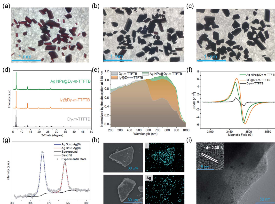
Fig. 3 Characterization of I_3^-@Dy-m-TTFTB and Ag NPs@Dy-m-TTFTB . The photographs of Dy- m -TTFTB (a), I_3^-@Dy-m-TTFTB (b) and Ag NPs@Dy-m-TTFTB (c) crystals. (d) Observed powder X-ray diffraction patterns for these three samples. (e) The solid-state absorption spectra of these three samples. (f) The EPR spectra of solid-state samples of Dy- m -TTFTB, I_3^-@Dy-m-TTFTB , and Ag NPs@Dy-m-TTFTB at 110 K. (g) The XPS spectra of Ag 3d of Ag NPs@Dy-m-TTFTB . (h) Elemental mapping of I_3^-@Dy-m-TTFTB and Ag NPs@Dy-m-TTFTB crystals under SEM/EDX. (i) HRTEM images of Ag NPs@Dy-m-TTFTB .
