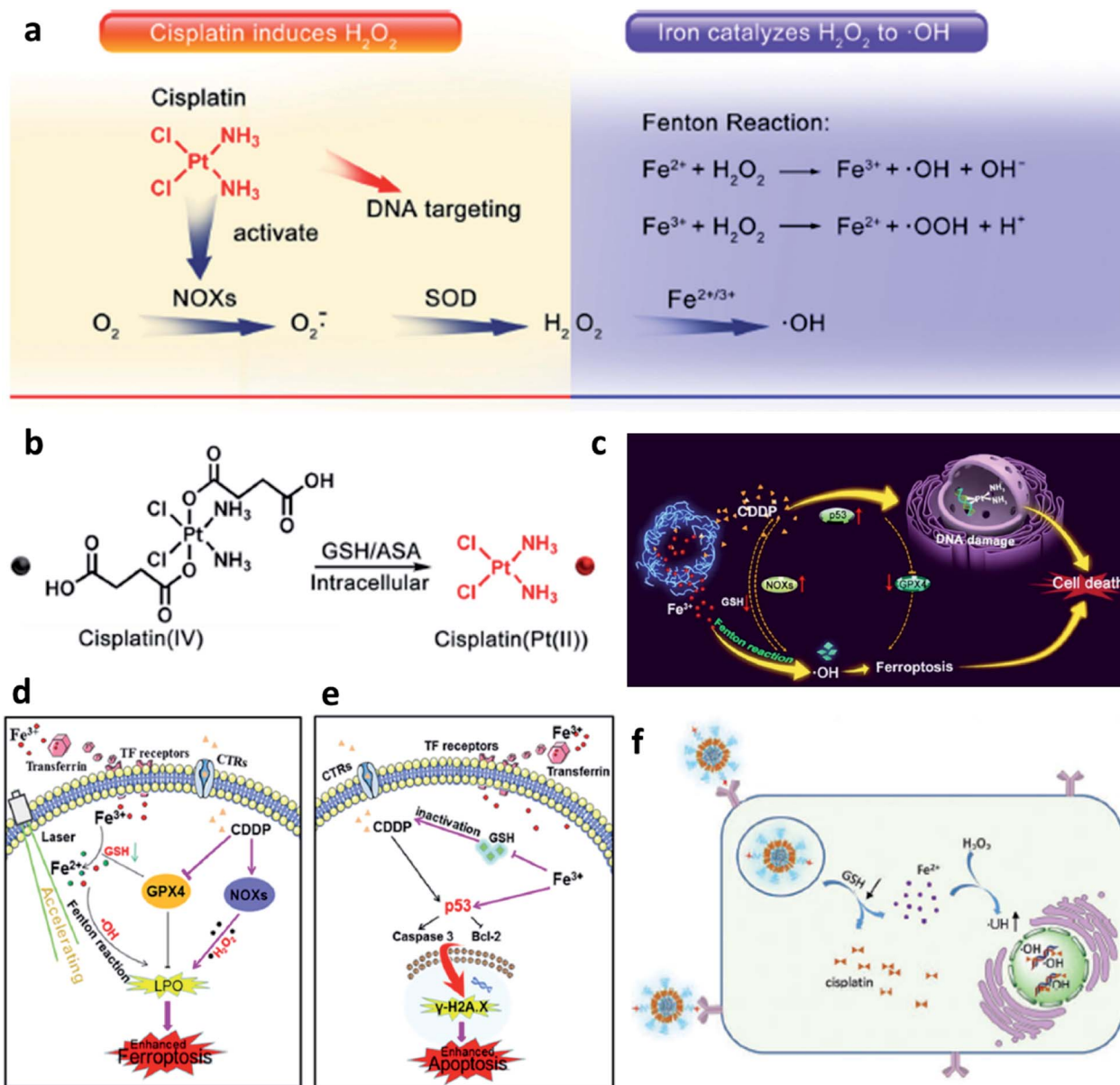
Fig. 6 (a) Cisplatin(Pt(II)) activates nicotinamide adenine dinucleotide phosphate (NADPH) oxidase (NOX), which can catalyze the formation of superoxide ( O_2^{\cdot-} ) and H_2O_2 from oxygen, iron ions catalyze the Fenton reaction to convert H_2O_2 into cytotoxic \cdot OH . (b) Cisplatin(IV) can be turned into cisplatin(Pt(II)) by reacting with intracellular GSH. Reproduced with permission from ref. 46. Copyright 2017, American Chemical Society. (c) Schematic illustration of synergistic therapy by combining cisplatin and Fe-based nanomaterials along with consuming the GSH. (d) Schematic illustration of cisplatin-enhanced CDT via adjusting relevant proteins. (e) Schematic illustration of CDT in CDDP-induced anticancer therapy. Reproduced with permission from ref. 47. Copyright 2020, American Chemical Society. (f) Schematic illustration of GSH consumption induced synergistic cisplatin release and \cdot OH generation and \cdot OH enhanced DNA damage. Reproduced with permission from ref. 48. Copyright 2020, Wiley-VCH.
