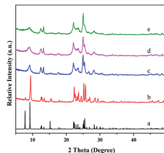
Fig. 1 XRD patterns of simulated FER (a), as-synthesized C-FER (b) and SCM-37 zeolites with different SAR of 15 (c), 20 (d), 25 (e).
