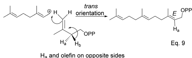
Scheme 6 Stereospecific dehydrogenation of farnesyl pyrophosphate (FPP) to form E and Z isomers.
