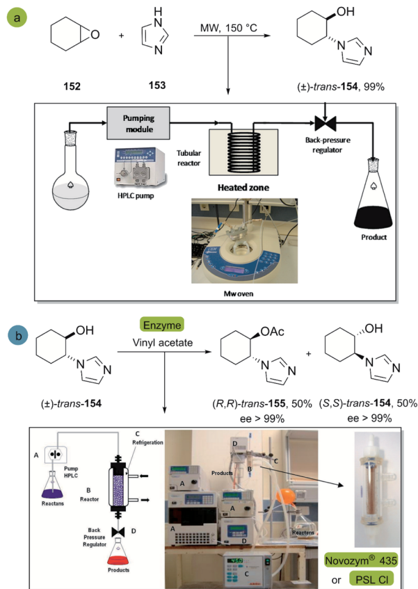
Scheme 22 Synthesis of trans -2-(1H-imidazol-1-yl)cyclohexanol (b) enantioselective acylation of ( \pm )- trans -2-(1H-imidazol-1-yl)cyclohexanol 154 with vinyl acetate catalyzed by Novozym® 435 or PSL-CI. This figure was used with permission. 100
