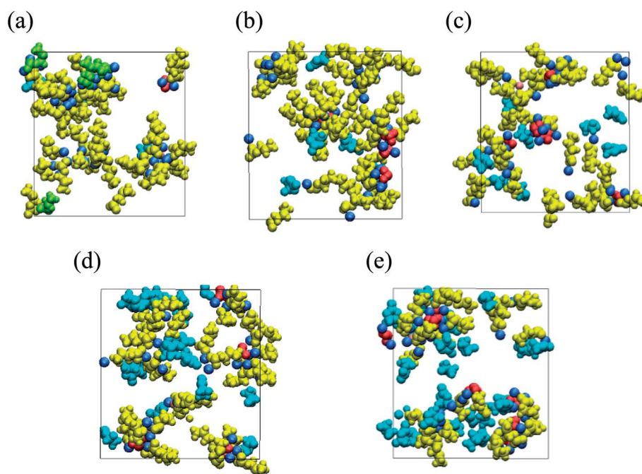
Fig. 9 Typical snapshot of SEI film at initial stage of formation (red, Na 2 CO 3 ; green, Na 2 DMBDC; dark yellow, NaPC; pink, NaF; cyan blue, FEC) in NaPF 6 /PC electrolyte solution containing (a) 1, (b) 3, (c) 5, (d) 7 and (e) 10 vol% of FEC additive concentration. 60 Copyright 2018, American Chemical Society.
