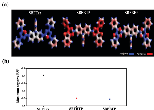
Fig. 7 (a) Electrostatic potential map of SBFTTrz, SBFBTP and SBFBFP (b) comparison of the maximum negative ESP of SBFTTrz, SBFBTP and SBFBFP.
