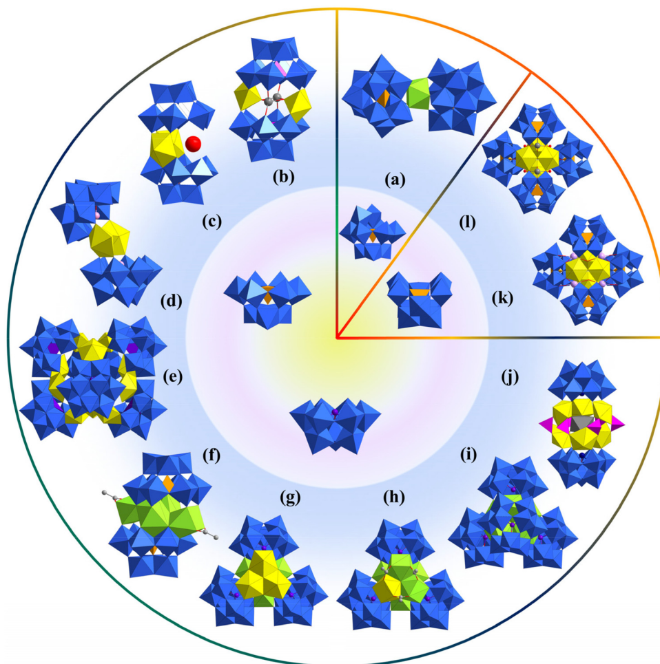
Fig. 1 View of Keggin-type U-hetero-POWs. (a) [\text{U}(\text{GeW}_{11}\text{O}_{39})_2]^{12-} ; typical structures of (b) \{\text{Na}_2(\text{UO}_2)_2(\text{XW}_9\text{O}_{34})_2\} ( X = \text{Si}, \text{P}, \text{Ge}, \text{As}^{\text{V}} ), (c) \{\text{M}_2(\text{UO}_2)_2(\text{XW}_9\text{O}_{34})_2\} ( \text{M} = \text{H}_2\text{O}, \text{NH}_4^+, \text{K}^+ ; X = \text{Si}, \text{P}, \text{As}^{\text{V}} ), (d) the “open” sandwich structure of \{(\text{UO}_2)_2(\text{H}_2\text{O})_2(\text{XW}_9\text{O}_{33})_2\} ( X = \text{As}^{\text{III}}, \text{Sb}^{\text{III}}, \text{Te}^{\text{IV}} ); (e) (\text{NH}_4)_{18}[(\text{NH}_4)_{12}(\text{UO}_2(\text{H}_2\text{O}))_6(\text{UO}_2(\mu_2\text{-H}_2\text{O}))_6(\alpha\text{-AsW}_9\text{O}_{34})_6] \cdot 74\text{H}_2\text{O} ; (f) [\text{U}_4(\mu_3\text{-O})_2(\text{SiW}_9\text{O}_{34})_2(\text{CH}_3\text{COO})_2]^{10-} ; (g) [(\text{U}^{\text{IV}})_5(\text{U}^{\text{VI}}\text{O})_{0.5}(\text{U}^{\text{VI}}\text{O})_{0.5}(\mu_3\text{-OH})_4(\mu_3\text{-O})_4\text{O}(\text{OAc})_2(\text{AsW}_9\text{O}_{33})_3]^{19-} ; (h) [(\text{U}^{\text{IV}})_3(\text{U}^{\text{VI}}\text{O})_3(\mu_3\text{-OH})_4(\mu_3\text{-O})_4(\text{AsW}_9\text{O}_{33})_3]^{15-} ; (i) [(\text{U}^{\text{IV}})_6(\mu_3\text{-OH})_4(\mu_3\text{-O})_4(\text{AsW}_9\text{O}_{33})_4]^{24-} ; (j) \{\text{Na}@\text{[(SbW}_9\text{O}_{33})_2(\text{UO}_2)_6(\text{PO}_3\text{OH})_6]\}^{17-} ; (k) [\{\text{K}(\text{OH}_2)\}_4(\text{UO}_2)_4(\text{OH})_2(\text{SiW}_{10}\text{O}_{36})_4]^{22-} ; (l) \{[\text{Na}(\text{OH}_2)]_4(\text{UO}_2)_4(\text{OH})_2(\text{SiW}_{10}\text{O}_{36})_4\}^{22-} . Color codes: W, blue; \text{U}^{\text{VI}} , yellow; \text{U}^{\text{IV}} , light green; Na, dark grey; K, lavender; P, magenta; Si and Ge, orange; As, purple; \text{Te}^{\text{IV}} , pink; \text{Sb}^{\text{III}} , dark blue; O, red; C, light grey.
