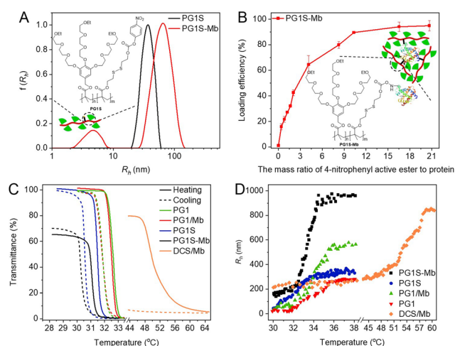
Fig. 2 (A) Plots of R_h from PG1S and PG1S-Mb . 25 °C, C = 0.05 mg \text{mL}^{-1} . The size polydispersities were 0.40 and 0.59, respectively. (B) Loading efficiency of PG1S for Mb at different concentrations. (C) Plots of transmittance vs. temperature for PG1S , PG1S-Mb , PG1 , PG1/Mb , and DCS/Mb . C = 2.5 mg \text{mL}^{-1} . (D) Plots of R_h for PG1S , PG1S-Mb , PG1 , PG1/Mb , and DCS/Mb between 30 and 60 °C, respectively. C = 0.05 mg \text{mL}^{-1} .
