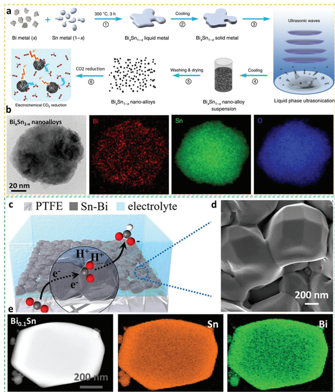
Fig. 6 (a) Schematics of the experimental steps to fabricate Bi x Sn 1-x nanoalloy electrocatalysts for CO 2 RR applications. (b) STEM-EDX mapping images of the Bi x Sn 1-x nanoalloy electrocatalysts. 2 This figure has been adapted from ref. 2 with permission from the Springer Nature, copyright 2019. (c) Schematic illustration of Bi 0.1 Sn alloying electrocatalysts on a polytetrafluoroethylene (PTFE) gas diffusion layer. (d) SEM image of Bi 0.1 Sn alloying electrocatalysts. (e) STEM-EDS mapping images of the Bi 0.1 Sn alloying electrocatalyst. 18 This figure has been adapted from ref. 18 with permission from the Springer Nature, copyright 2021.
