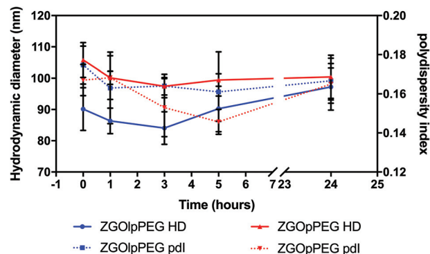
Fig. 4 Evolution of the hydrodynamic diameter (continuous line) and polydispersity index (dashed line) of ZGOlpPEG (blue) and ZGOPEG (red) in 5% glucose injection medium ( n = 3 ).
