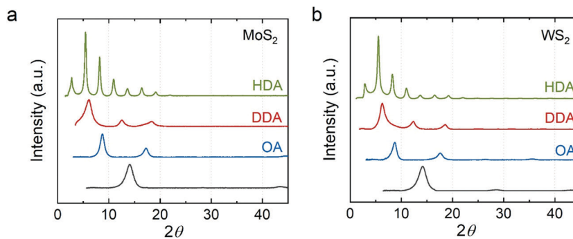
Fig. 3 XRD of the n -alkylamine intercalated (a) MoS 2 and (b) WS 2 . Green: hexadecylamine-intercalated; red: dodecylamine-intercalated; blue: octylamine-intercalated; dark gray: restacked.
