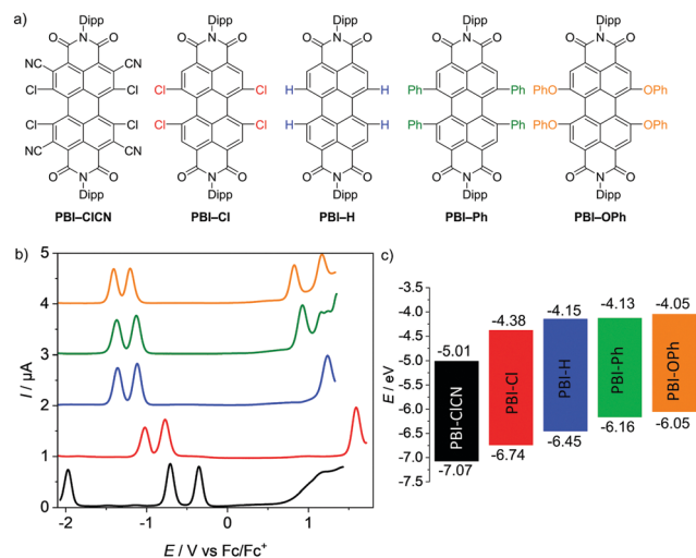
Fig. 1 (a) Molecular structures of the PBIs with bulky 2,6-diisopropylphenyl (Dipp) imide substituents investigated by electrochemical reduction. (b) Square wave voltammograms of PBI-C1CN (black), PBI-Cl (red), PBI-H (blue), PBI-Ph (green) and PBI-OPh (orange). Measurements were performed using DCM solutions ( c_0 = 2 \times 10^{-4} M) at room temperature, using TBAHFP (0.1 M) as electrolyte (scan rate 100 \text{ mV s}^{-1} , SW amplitude 25 mV, SW frequency 15 Hz). (c) Schematic diagram of the electrical band gaps of the investigated PBIs (energy level of \text{Fc}/\text{Fc}^+ with respect to the vacuum level = -5.15 \text{ eV} ). 15
