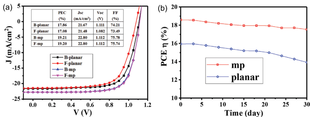
Fig. 11 (a) J–V graphs obtained of the planar SnO 2 and mp SnO 2 PSCs from under backward and forward voltage scanning. (b) PCEs of the planar SnO 2 and mp SnO 2 PSCs monitored every 3 d; the measurement was performed under AM 1.5G with input solar power P_{in} of 100 mW cm −2 . Reprinted with permission from ref. 224. Copyright 2018 John Wiley and Sons.
