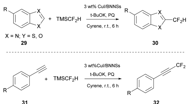
Scheme 7 Difluoromethylation of heteroarenes ( 29 ) and terminal alkynes ( 31 ) using Cyrene as the solvent. All reactions were performed with 29 or 31 (1.0 equiv.), \text{TMSCF}_2\text{H} (2.0 equiv.), catalyst (10 mg), t -BuOK (3 equiv.), and 9,10-phenanthrenequinone (PQ) (1.2 equiv.).
