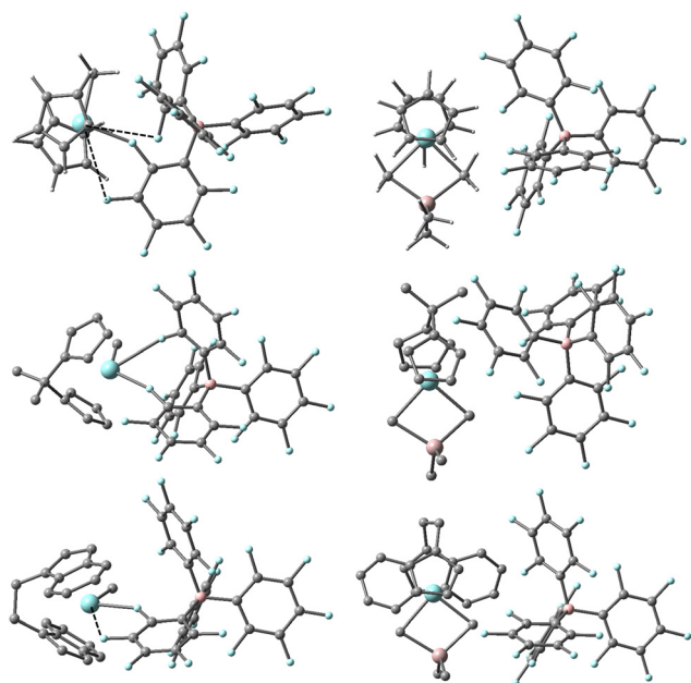
Fig. 3 Most stable structures of [L_2ZrMe][B(C_6F_5)_4] ( L_2 = Cp_2 , 45 Me_2CCp_2 and EBI , left) and [L_2ZrMe_2AlMe_2][B(C_6F_5)_4] (right) based on Gibbs energy ( \Delta G_{\text{qh-tr}} ) at the M062-X/TZVP level of theory. Zr and F in blue, Al and B in pink, C in grey, H omitted from lower two structures for clarity. Long Zr–F contacts are shown as dashed lines.
