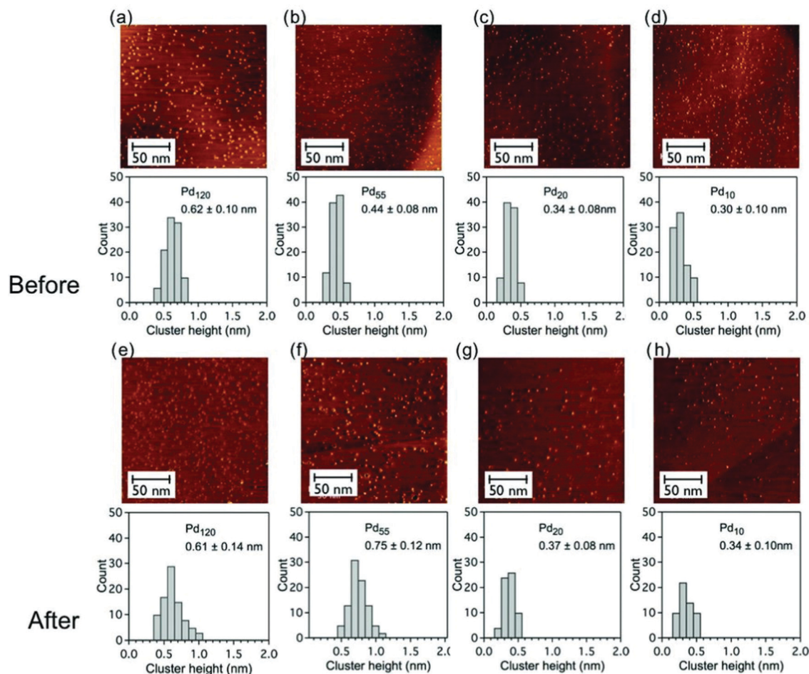
Fig. 3 Constant current STM images (200 × 200 nm 2 , 0.4 nA, 0.4 V) of graphite-supported size-selected Pd N clusters (N = 120, 55, 20 and 10, low coverage) and histograms of the cluster height distributions before and after catalytic reaction at reactant ratio of C 6 H 12 :O 2 = 1 : 10; (a–d) as-deposited clusters before catalytic measurements and (e–h) after reaction catalytic measurements. The mean height of the cluster is given in each case. Adapted from ref. 103 with permission from Taylor & Francis.
