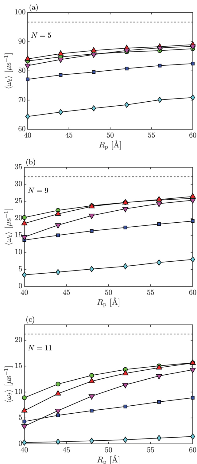
Fig. 8 The capsule's tumbling rate, \langle\omega_t\rangle , for R_p = 40 \text{ Å} to 60 \text{ Å} for parameters: (▽) V_m = -1 \text{ V} , q_i = -2e ; (Δ) V_m = -1 \text{ V} , q_i = -1e ; (○) q_i = 0 ; (□) V_m = 1 \text{ V} , q_i = -1e ; (◊) V_m = 1 \text{ V} , q_i = -2e ; dashed line is for q_i = 0 in free space (outside of the pore). The capsule lengths studied include (a) N = 5 , (b) N = 9 , and (c) N = 11 .
