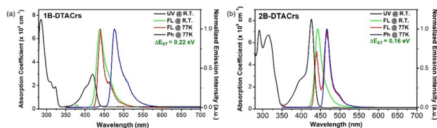
Fig. 3 Photophysical properties of (a) 1B-DTACr and (b) 2B-DTACr in toluene solution ( 10^{-5} M) at room temperature and 77 K ( \lambda_{\text{exc}} = 280 nm and 320 nm for time-resolved and steady-state emission, respectively).
