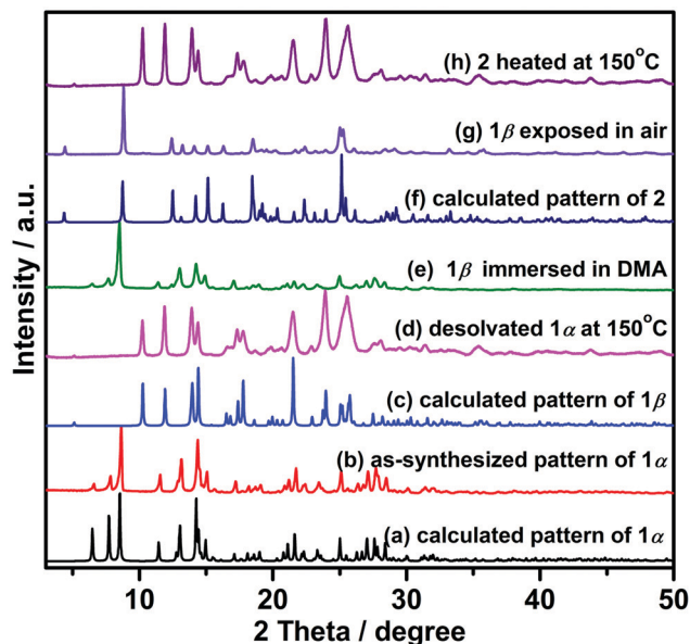
Fig. 3 PXRD patterns of (a) 1\alpha calculated from SCXRD data, (b) as-synthesized 1\alpha at room temperature, (c) 1\beta calculated from SCXRD data, (d) desolvated 1\alpha at 150\text{ }^\circ\text{C} , (e) 1\beta immersed in DMA for 1 day, (f) calculated 2 from SCXRD data, (g) 1\beta exposed to humid air (ca. 45% RH), and (h) dehydrated 2 at 150\text{ }^\circ\text{C} .
