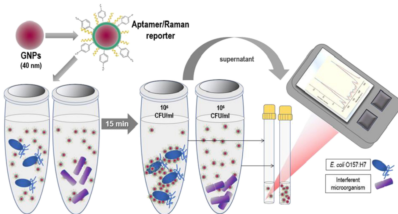
Fig. 8 Schematic illustration of the detection mechanism proposed for aptamer-based whole cell detection of E. coli O157:H7. The image is reprinted from Díaz-Amaya et al. , 120 Copyright (2019), with permission from Elsevier.
