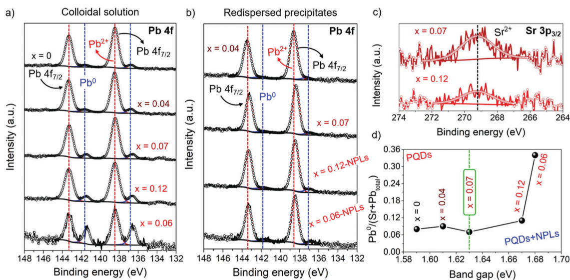
Fig. 3 High-resolution (HR) XPS spectra of (a and b) Pb 4f, (c) XPS Sr 3p 3/2 and (d) calculated metallic Pb 0 -to-(Sr + Pb total ) ratio for (a, c and d) \text{FAPb}_{1-x}\text{Sr}_x\text{I}_3 PQDs colloidal solutions, and (b) their corresponding redispersed precipitates.
