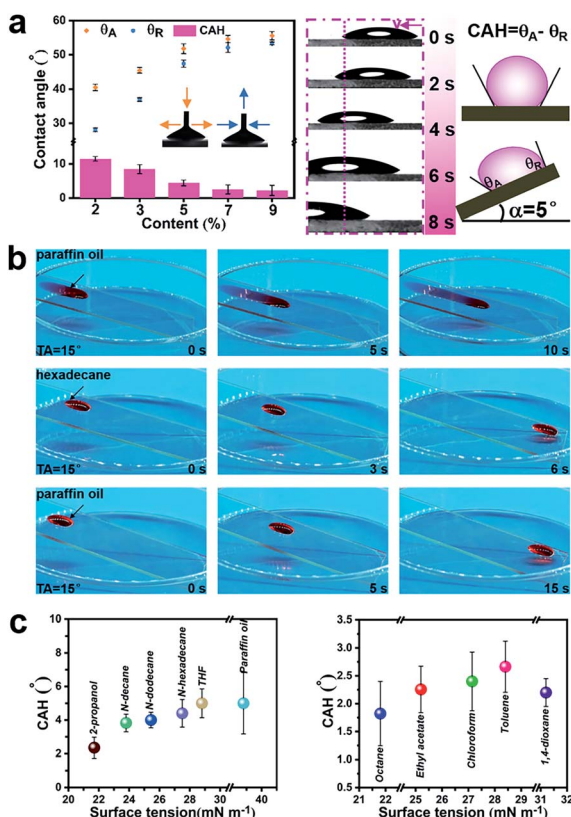
Fig. 6 (a) \theta_{adv} , \theta_{rec} and CAH ( \Delta\theta ) of the hexadecane on the sample coatings; time-sequence images of the 10 \mu L hexadecane droplet sliding on the C-5 coating with a tilt angle (TA) of 5^\circ . (b) Surface liquid repellence of C-5 against hexadecane and paraffin oil (dyed by oil red, tilted angle of 15^\circ ). (c) CAH of different organic liquids on glass slides coated with C-5 coatings.
