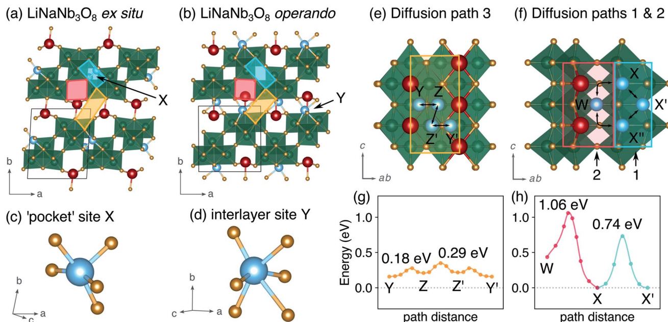
Fig. 9 Structures obtained from DFT calculations for intercalation to (\text{LiNaNb})_3\text{O}_8 . (a) Ground-state structure with \text{Li} in five-fold coordinate 'pocket' sites within \text{Nb}_3\text{O}_8 layers, corresponding to the structure from ex situ XRD analysis. (b) Metastable structure with \text{Li} in distorted octahedral interlayer sites, corresponding to the structure from operando XRD analysis. Figures (c) and (d) show detail of the \text{Li} geometry from (a) and (b) respectively. Red, blue, and gold quadrilaterals indicate pathways along the square channels, within the \text{Nb}_3\text{O}_8 layers, and within the interlayer space, respectively. (e) Diffusion pathway 3 in the interlayer space. (f) Diffusion paths 1 and 2 within the \text{Nb}_3\text{O}_8 layers. Calculated activation barriers for (g) diffusion along pathway 3 and (h) along paths 1 and 2.
