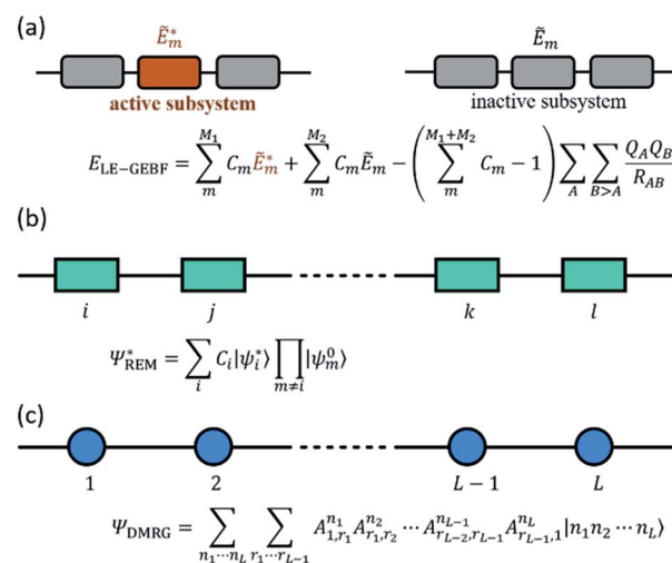
Fig. 4 Schematic illustration of (a) LE-GEFB subsystems, (b) REM wavefunction, and (c) DMRG wavefunction. The rectangle in (b) denotes a molecular fragment or block and |\psi_i^0\rangle and |\psi_i^*\rangle are the wavefunctions of its ground and excited states respectively with C_i being the configuration coefficient. The circle in the bottom denotes a molecular orbital or a vibrational mode, and |n_i\rangle represents its local basis with A^{n_i} being MPS matrices.
