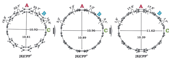
Fig. 5 Optimized geometries along with selected geometrical parameters for \mathbf{1}^0 , \mathbf{1}^{2-} , and \mathbf{1}^{4-} (PBE0/cc-pVTZ).
