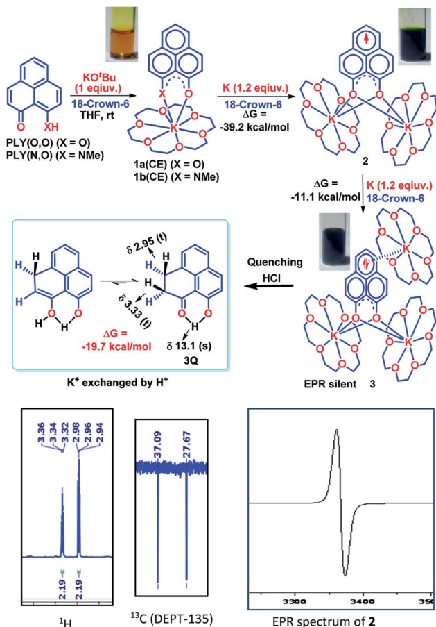
Scheme 1 Preparation of the PLY–K complexes (1a(CE) and 1b(CE), 12\pi \text{ e}^- species) and consecutive one electron reduction by K to generate mono-reduced 13\pi \text{ e}^- species (2) and doubly reduced 14\pi \text{ e}^- species (3), respectively; quenching the 14\pi \text{ e}^- species by replacing all \text{K}^+ ions with \text{H}^+ ions through HCl treatment; (insets: EPR spectrum of 2 and selected part of ^1\text{H} and ^{13}\text{C} (DEPT-135) NMR spectra of 3Q).
