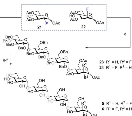
Scheme 2 Preparation of fluorinated maltotetraose cores 5 and 6 . Conditions: (a) Ac 2 O, DMAP, pyridine, 4 h, RT, 88%. (b) 4-Methylbenzenethiol, BF 3 ·OEt 2 , CH 2 Cl 2 , 23 h, RT, 78%. (c) (1) NaOMe, MeOH, 2 h, RT, 91%; (2) NaH, BnBr, TBAL, DMF, 20 h, RT, 77%. (d) NIS, BF 3 ·OEt 2 , CH 2 Cl 2 , 15 min, RT, 23 : 21%, 24 : 25%. (e) Pd/C, H 2 , MeOH, EtOAc, 24 h, RT; (f) NaOMe, MeOH, 8 h, RT, 5 : 88%, 6 : 67% over two steps.
