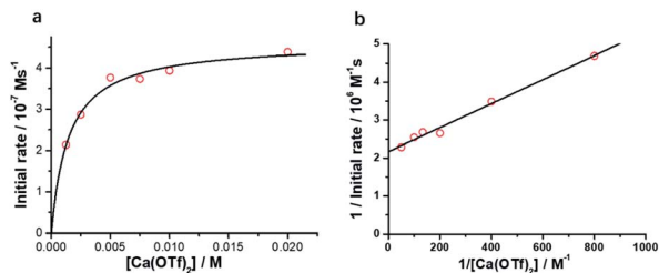
Fig. 3 Effects of [Ca(OTf) 2 ] on cyclohexane oxidation by RuO 4 - in CH 3 CN. Conditions: [ n Pr 4 N][RuO 4 ] (0.01 M), cyclohexane (1.0 M) in CH 3 CN at 23 °C. (a) Plot of initial rate vs. [Ca(OTf) 2 ]. (b) Plot of 1/initial rate vs. 1/[Ca(OTf) 2 ] (slope = (3.16 ± 0.15) × 10 3 , y-intercept = (2.16 ± 0.06) × 10 6 , r = 0.988).
