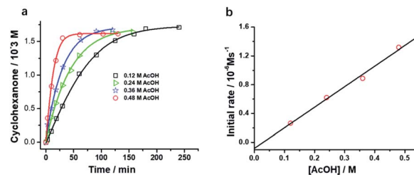
Fig. 4 (a) Effects of CH 3 CO 2 H on cyclohexane oxidation by RuO 4 - in CH 3 CN. Conditions: [ n Pr 4 N][RuO 4 ] (0.01 M), cyclohexane (1.0 M) in CH 3 CN at 23 °C. (b) Plot of initial rate versus [AcOH]. (slope = (2.72 ± 0.13) × 10 -6 , y-intercept = -(3.33 ± 3.82) × 10 -8 , r = 0.9908).
