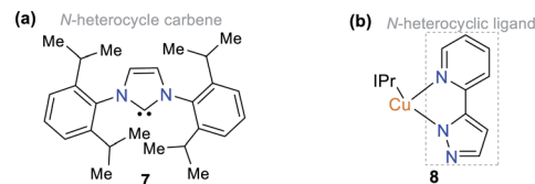
Fig. 3 Structure of (a) ligand IPr 7 and (b) \text{Cu}(\text{I}) complex 8 .
