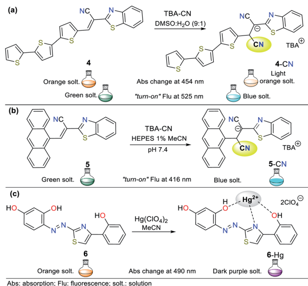
Fig. 2 Probes based on thiazoles for \text{CN}^- sensing in (a) \text{DMSO} : \text{H}_2\text{O} and (b) in HEPS solution (1% MeCN as a co-solvent), and (c) for \text{Hg}^{2+} recognition.
