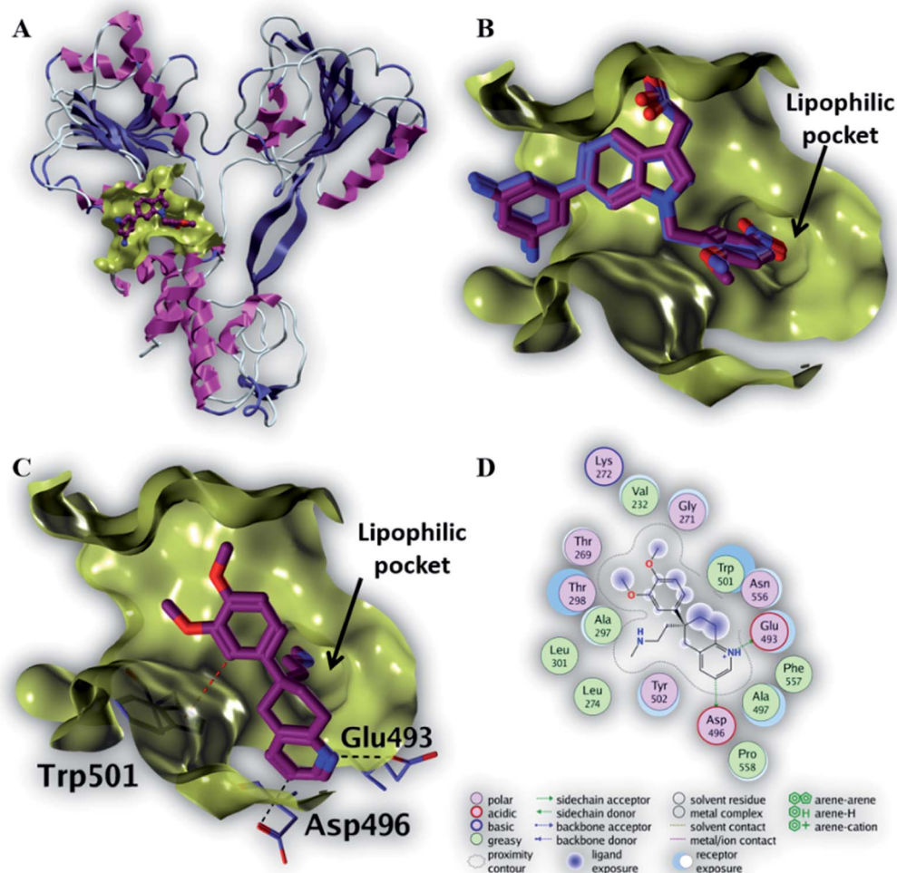
Fig. 5 The top-scoring docked pose of compound 6 to the HCV NS3 helicase active site (PDB code 4OKS) as predicted by MOE 2019.01. (A) An overview of the HCV NS3 helicase active site (B) comparison of modeled binding mode of the co-crystallized ligand (magenta stick model) and its superposed docking conformation (blue stick model). (C) Detailed binding mode of compound 6 (magenta stick model) displaying hydrogen bonds (black dashed line) with the key amino acid residue (blue stick model). (D) 2D depiction of compound 6 binding interactions with the key amino acid residues.
